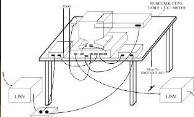
Figure 4.1.1. Generic Test set up for the Yeong Yang YY-55XX Personal Computer chassis
