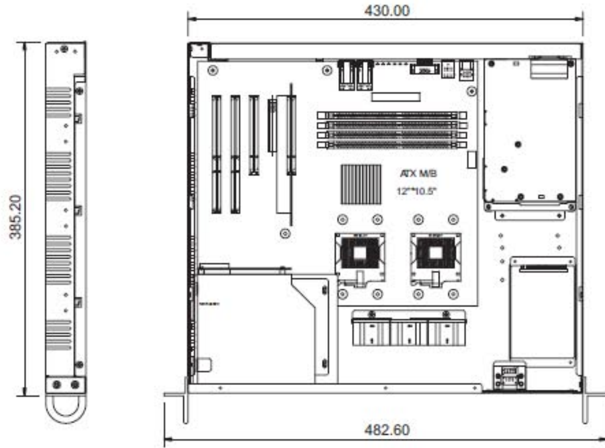
Left-side View
