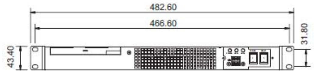
Front View-2
